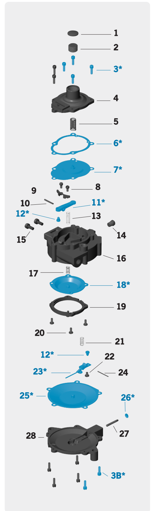
Note: Parts in blue are components of Repair Kit (N-RK-51A).
